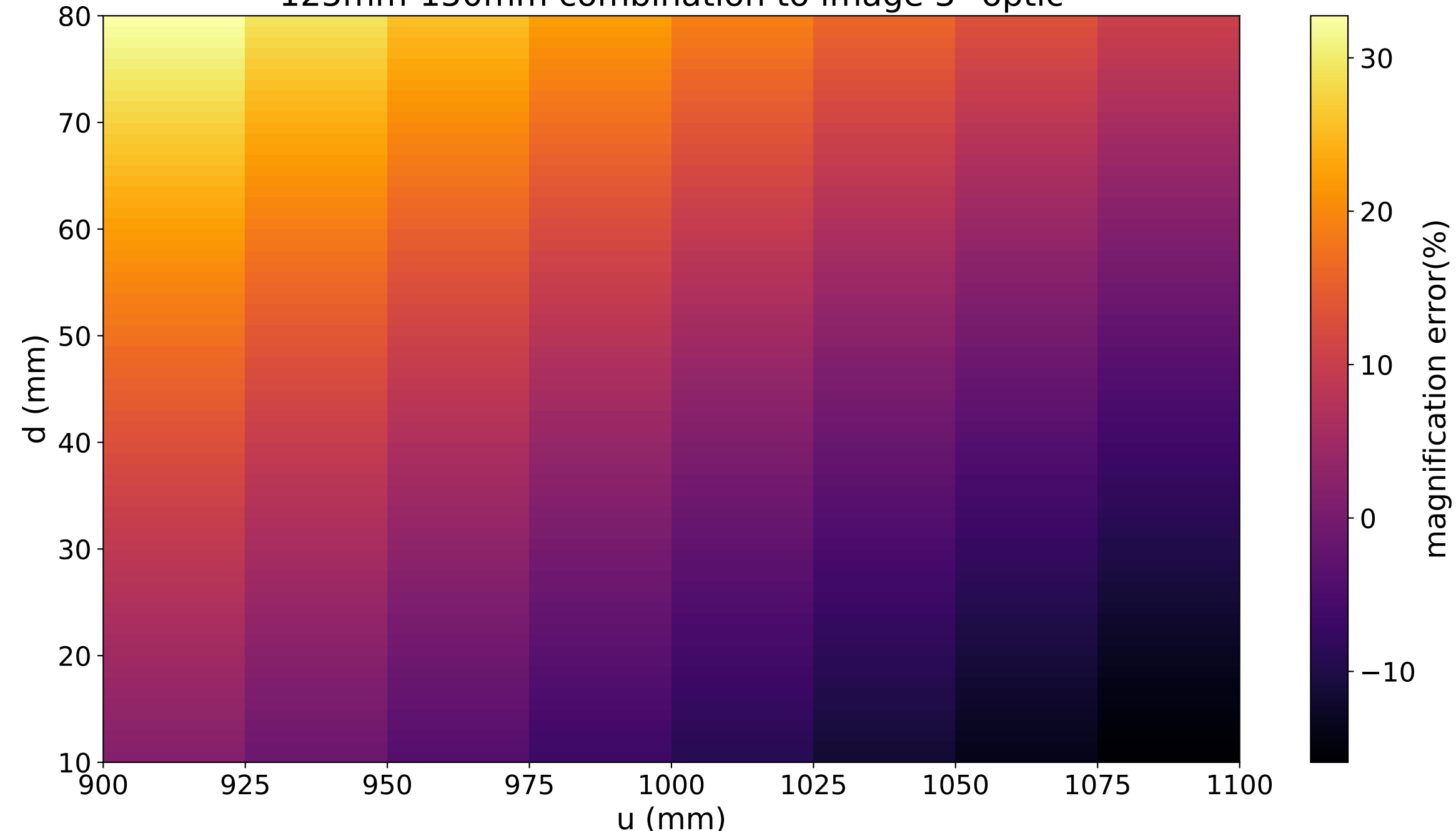
125mm-150mm combination to image 3" optic
