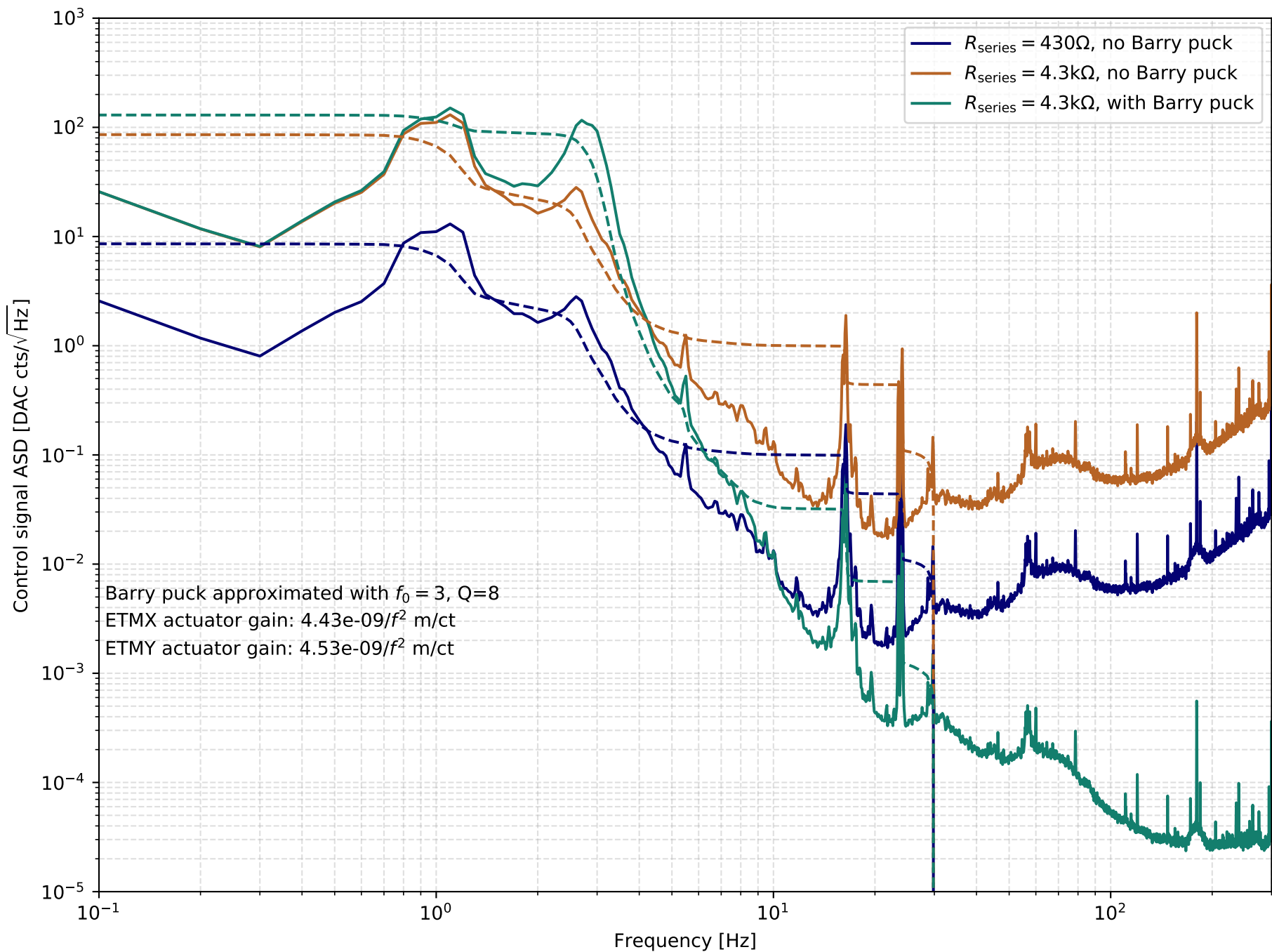
Projections of control signal required for DARM control
