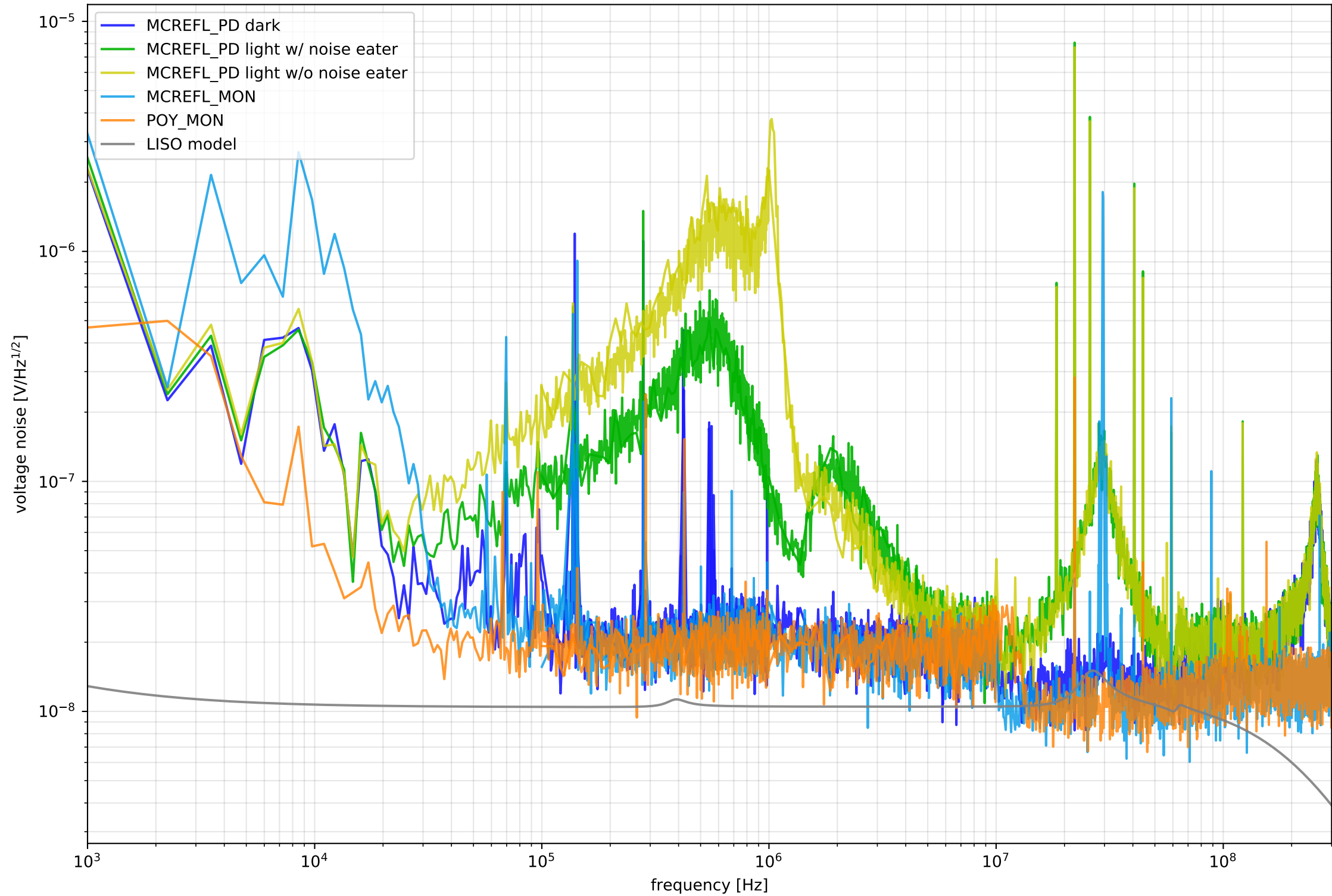
MC REFL PD Voltage Noise
