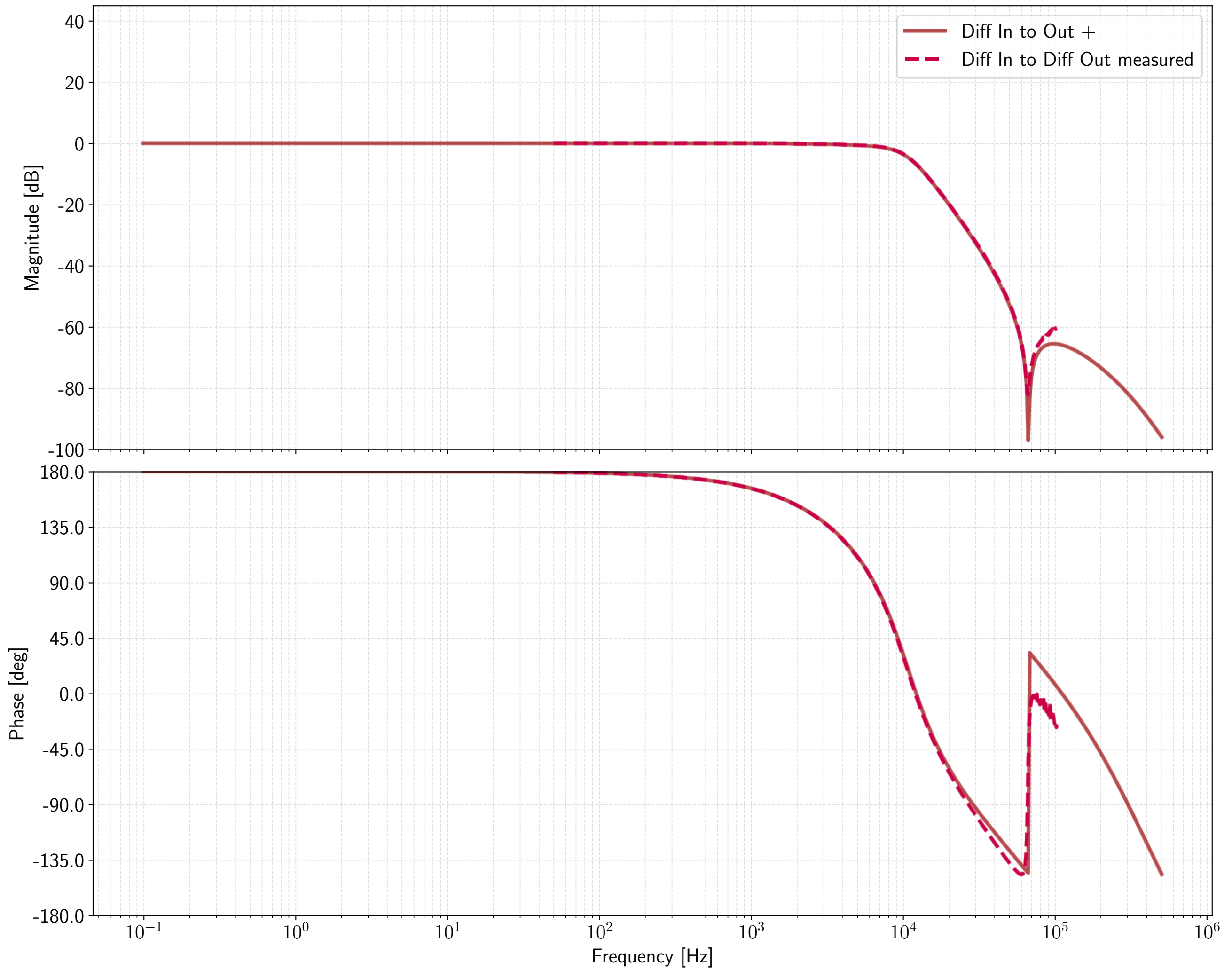
D070081 AA board V2 Transfer Function
