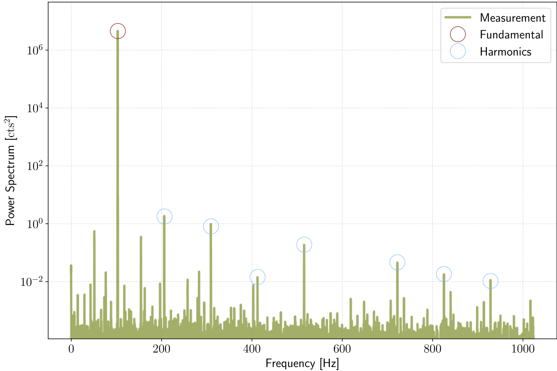
THD measurement, f_0 = 103.17 Hz, N = 8
