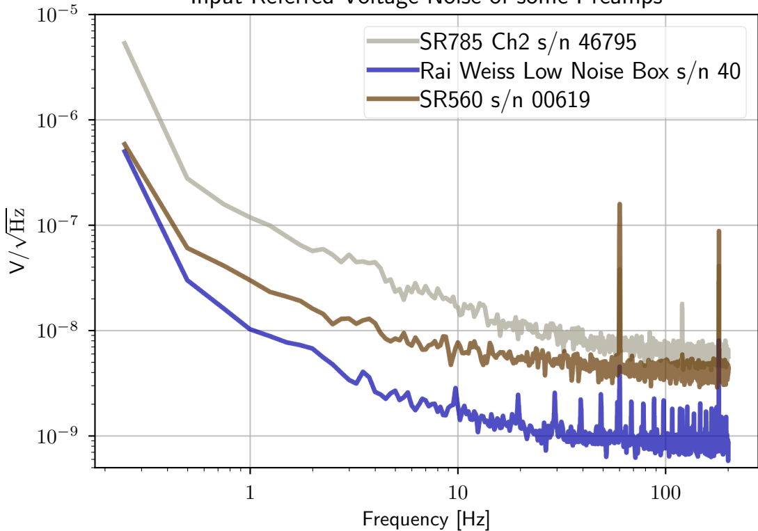
Input Referred Voltage Noise of some Preamps
