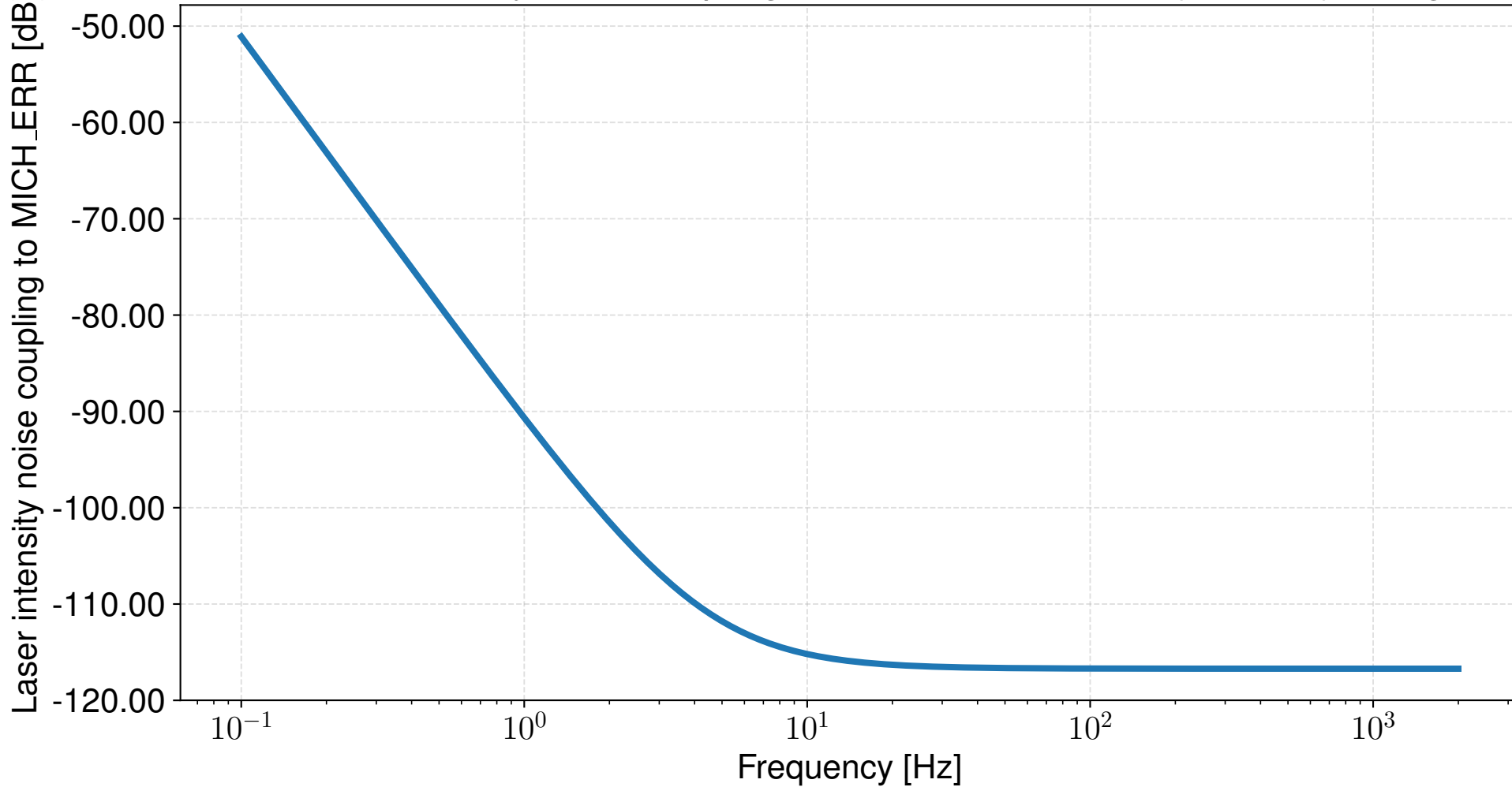
Modelled laser intensity noise coupling to MICH in 40m DRMI (no arms) configuration
