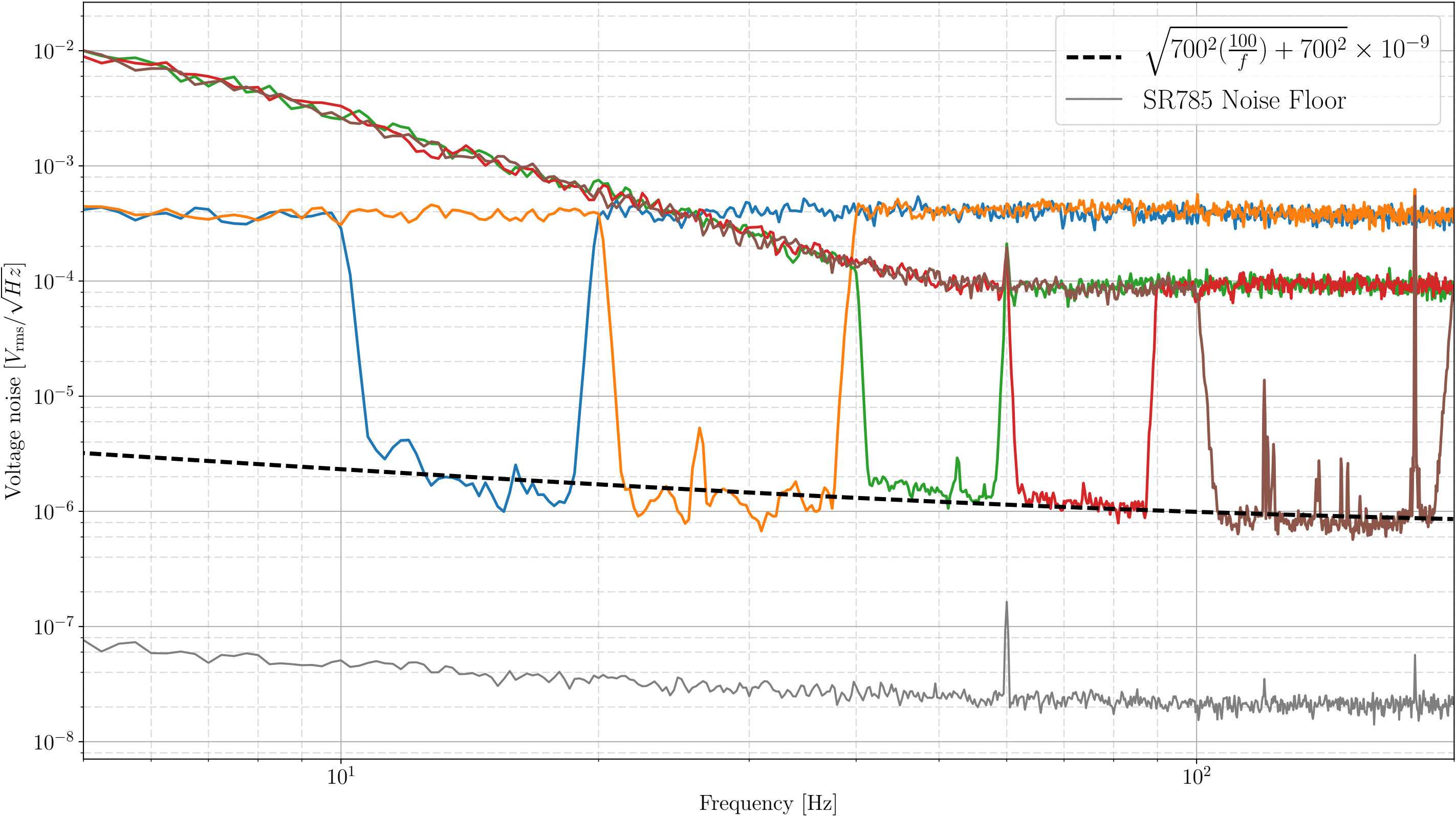
DAC Noise vs Frequency Model
