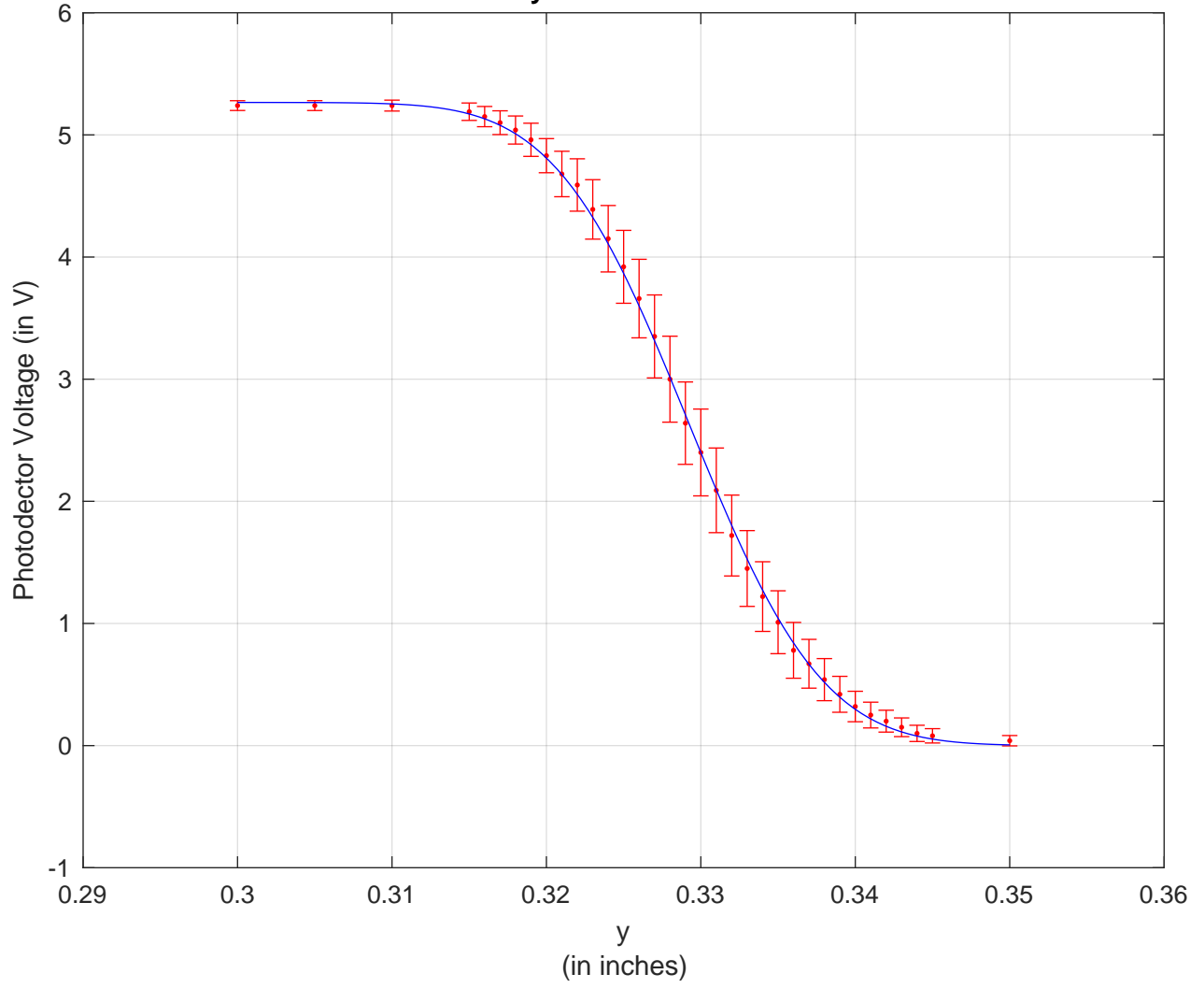
Beam y-Profile at z = 10cm
