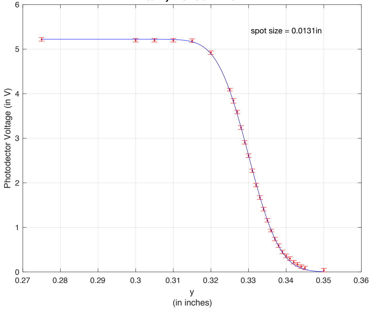
Beam y-Profile at z = 4cm
