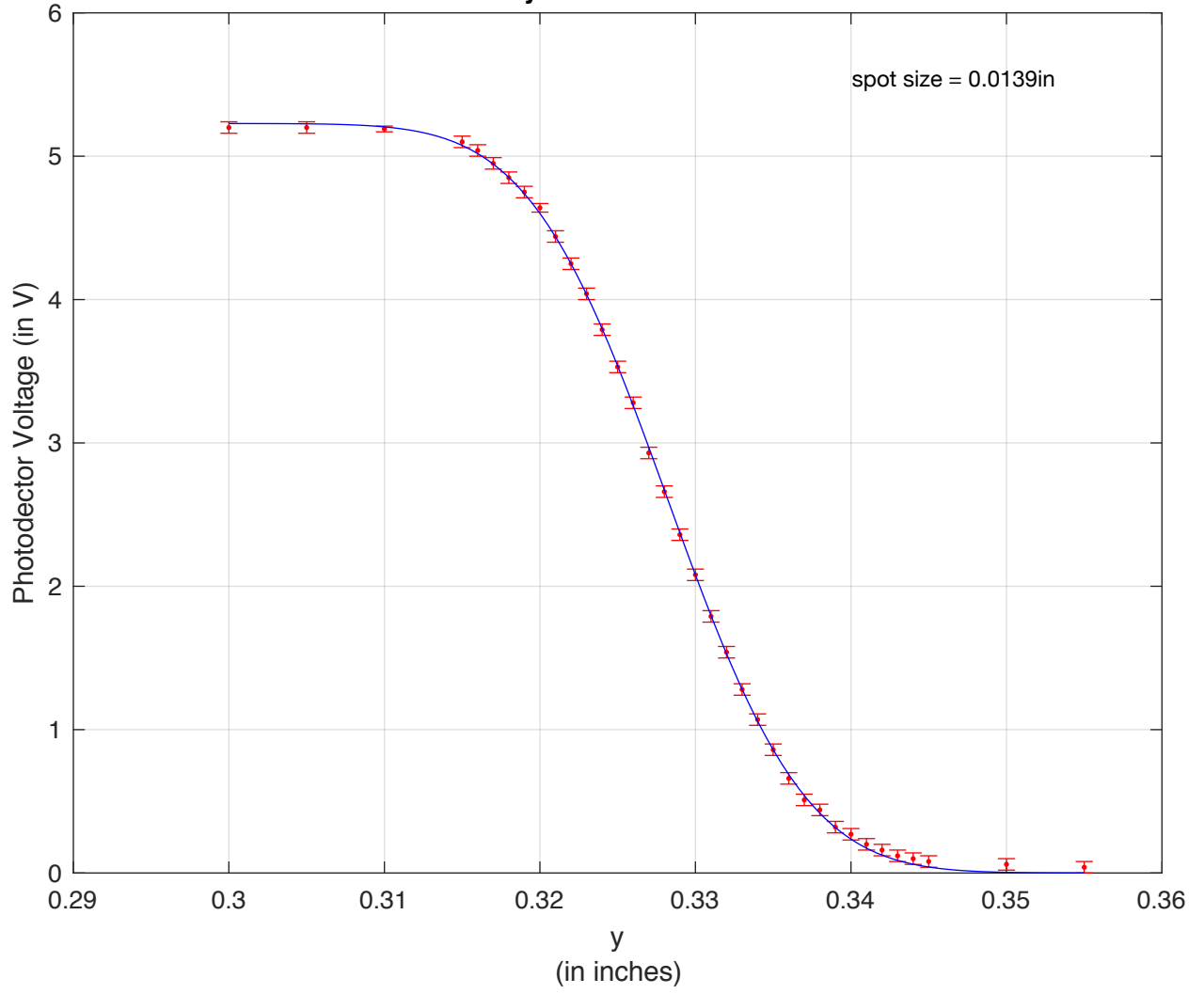
Beam y-Profile at z = 20cm
