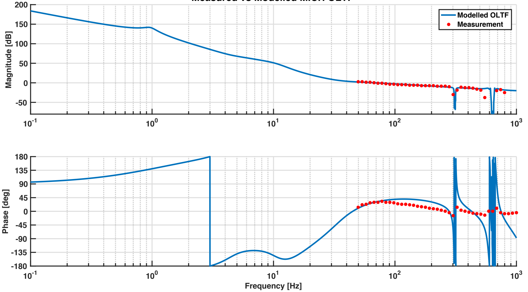
Measured vs Modelled MICH OLTF
