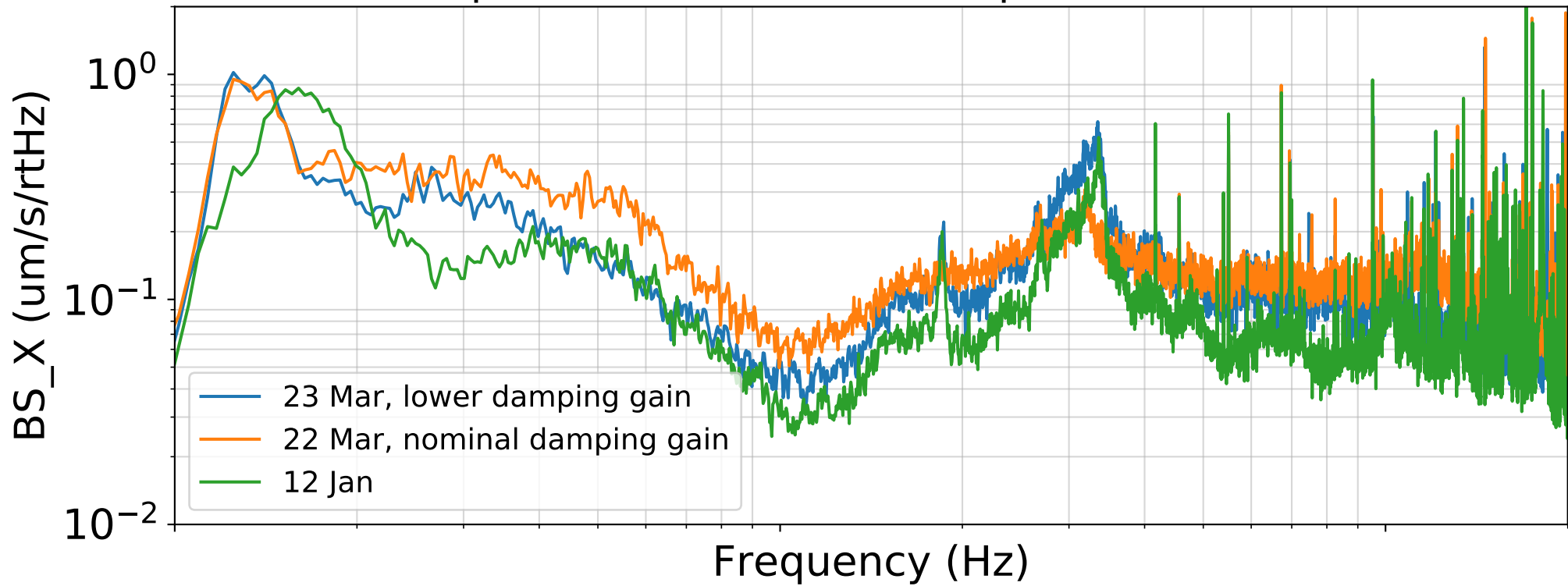
Comparison of seismometer spectra over dates
