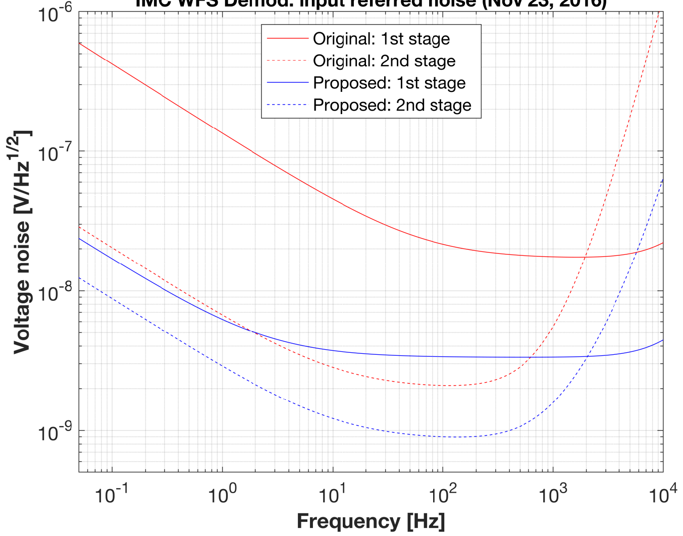
IMC WFS Demod: input referred noise (Nov 23, 2016)
