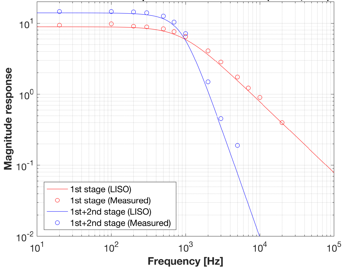
IMC WFS Demod: Response ~ measued & model (Nov 23, 2016)
