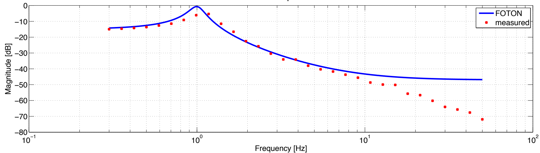
Measured Plant TF compared to modelled TF
