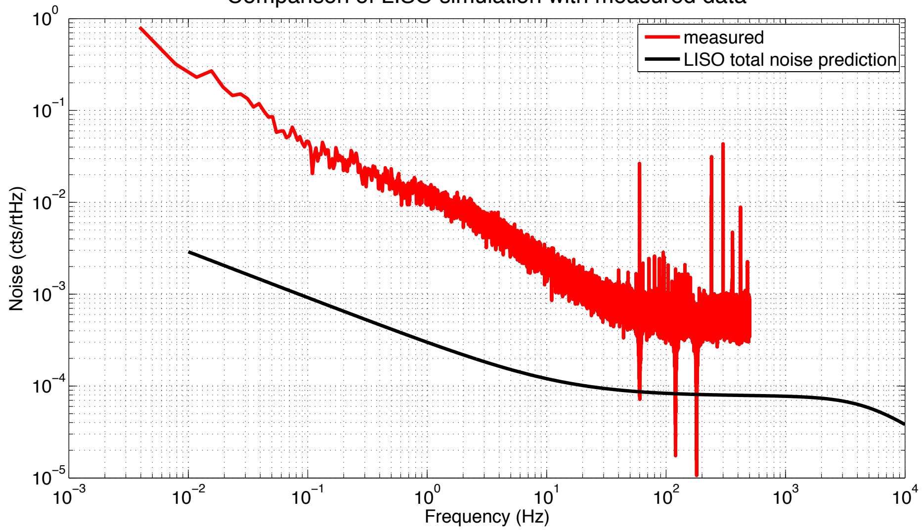
Comparison of LISO simulation with measured data
