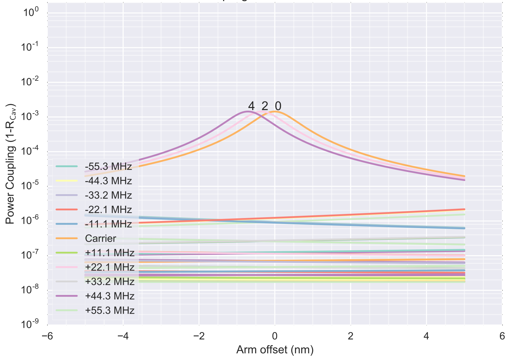
Power Coupling of HOMs into 40m Y Arm
