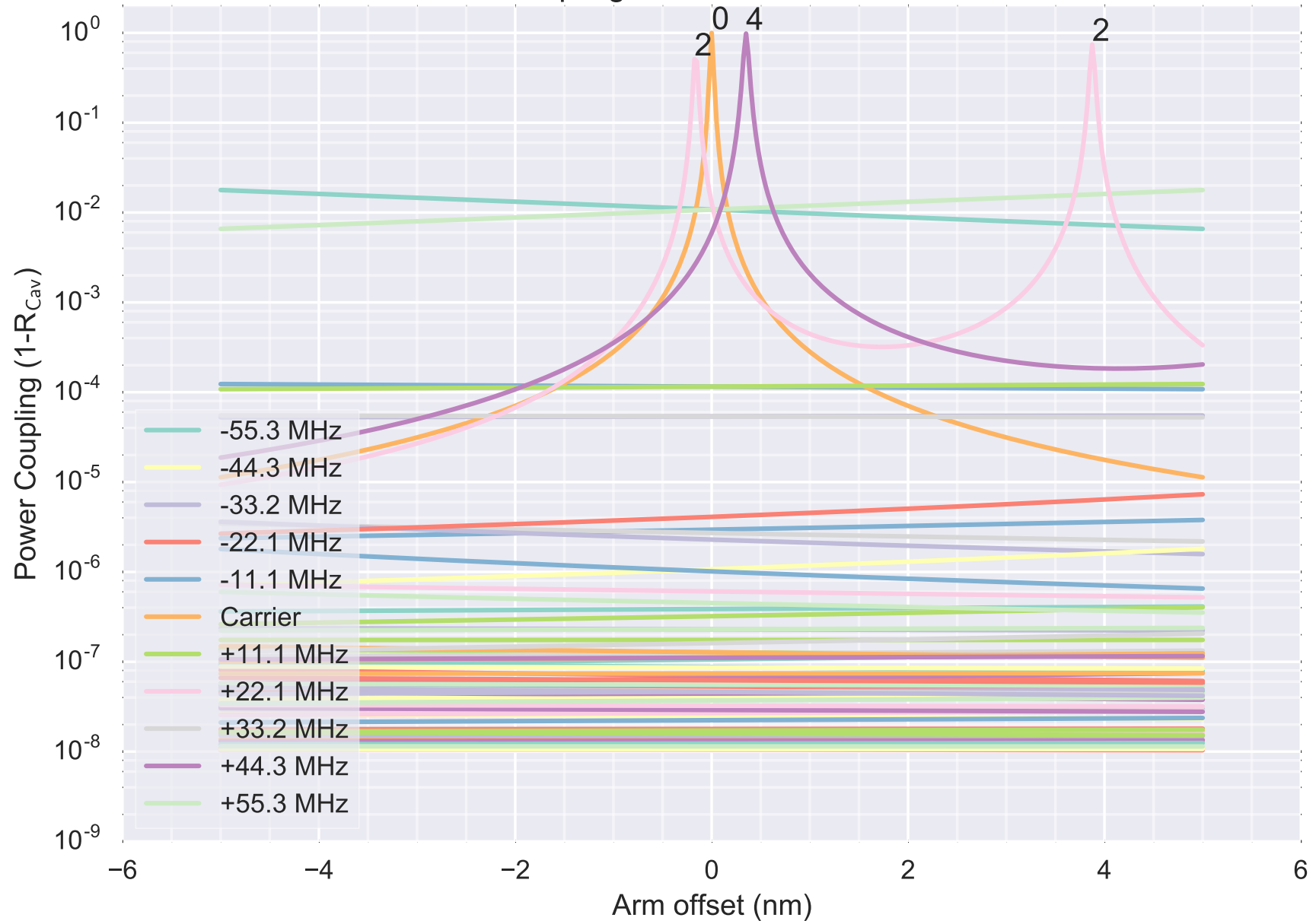
Power Coupling of HOMs into 40m DRFPMI
