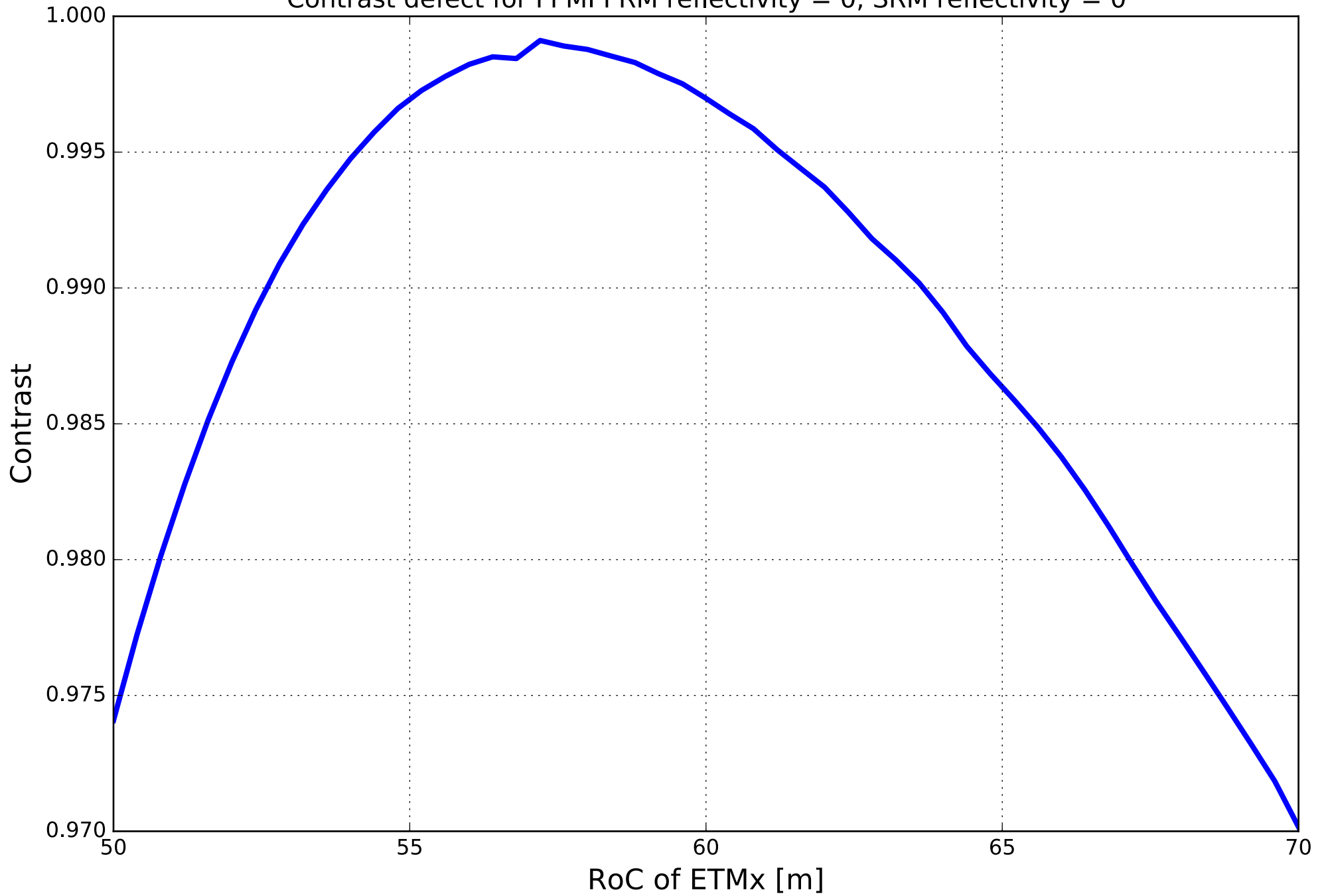
Contrast defect for FPMI PRM reflectivity = 0, SRM reflectivity = 0
