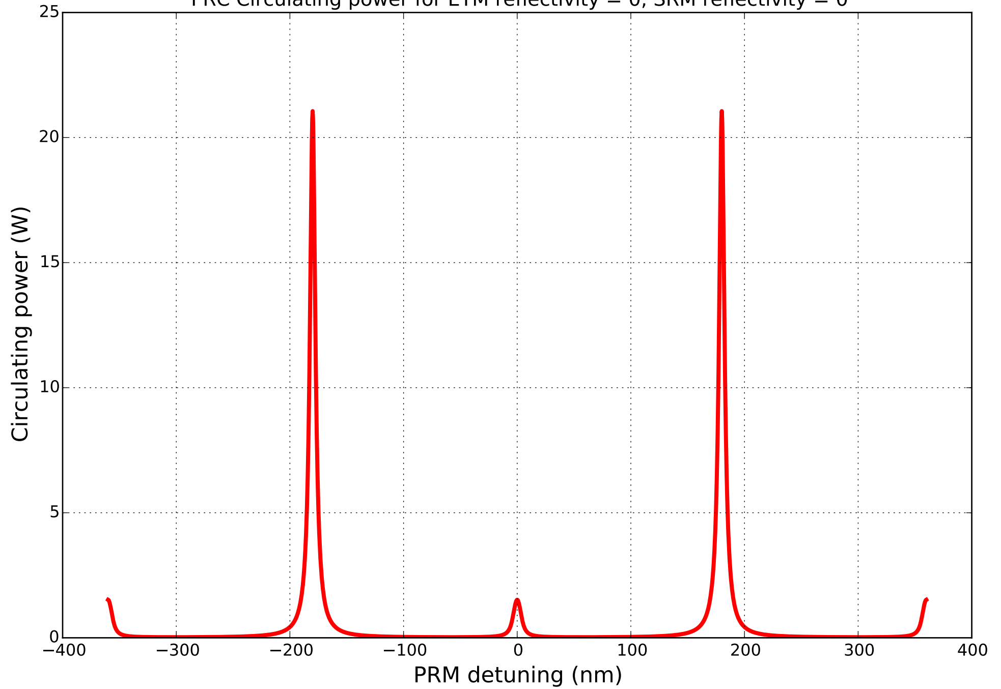
PRC Circulating power for ETM reflectivity = 0, SRM reflectivity = 0
