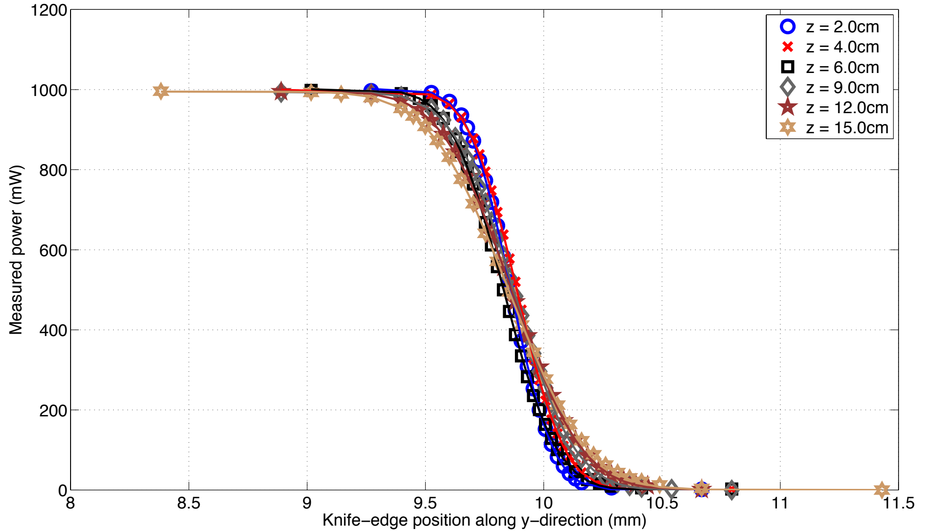
Beam profiling Innolight 1W NPRO – Knife-edge scans along y-direction
