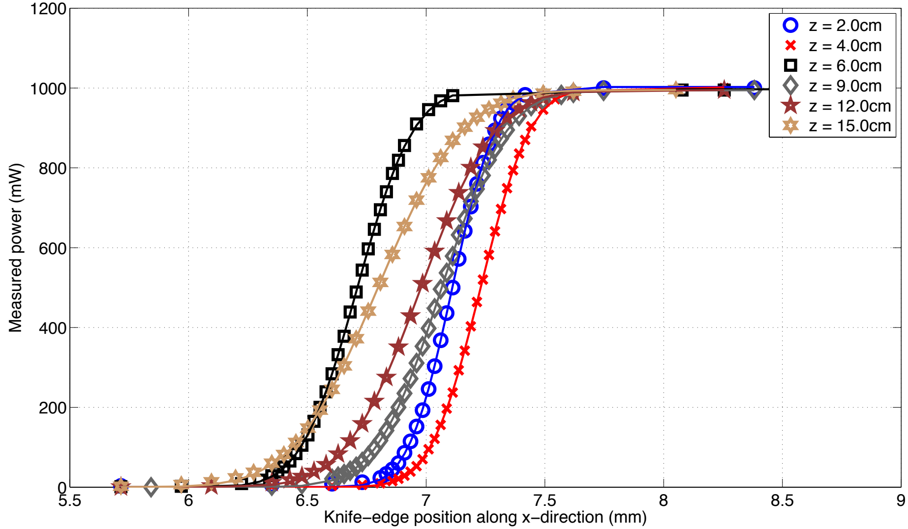
Beam profiling Innolight 1W NPRO – Knife-edge scans along x-direction
