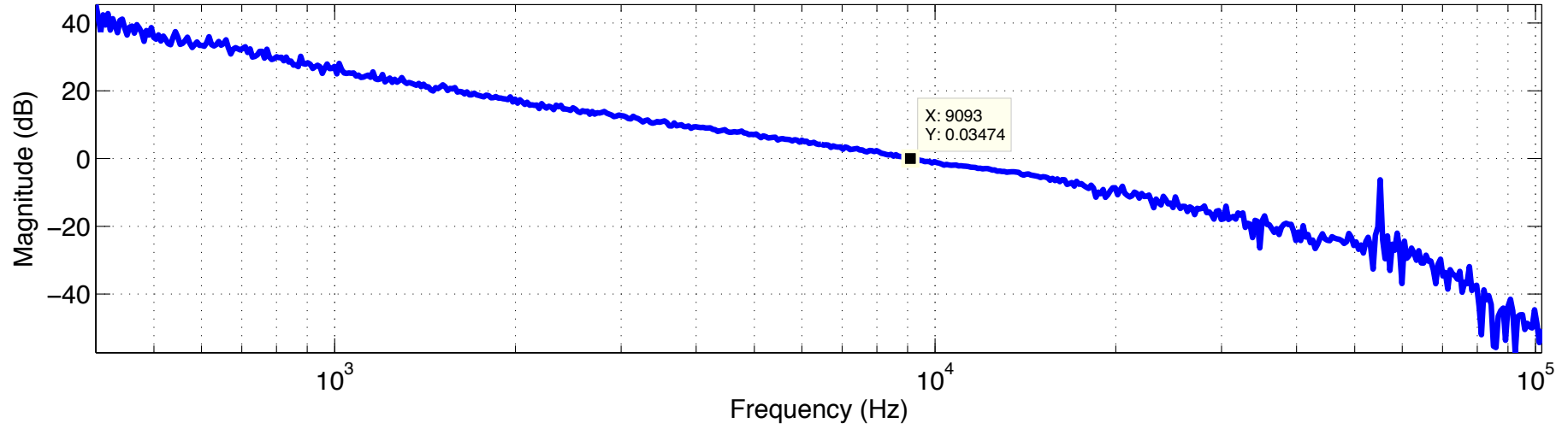
AUX PDH: X end OLTF
