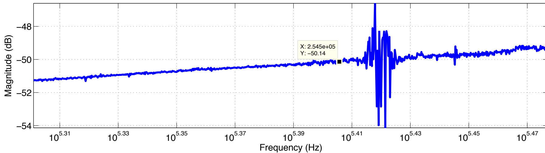
Transfer function from LO input of Pomona box to laser PZT
