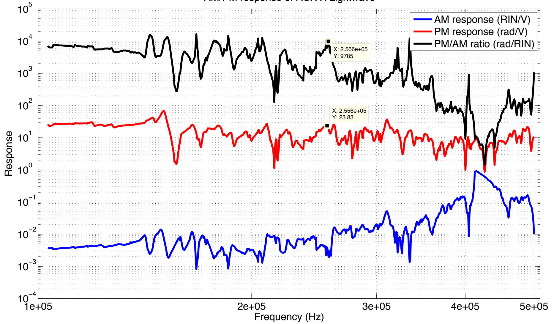
AM/PM response of AUX X Lightwave
