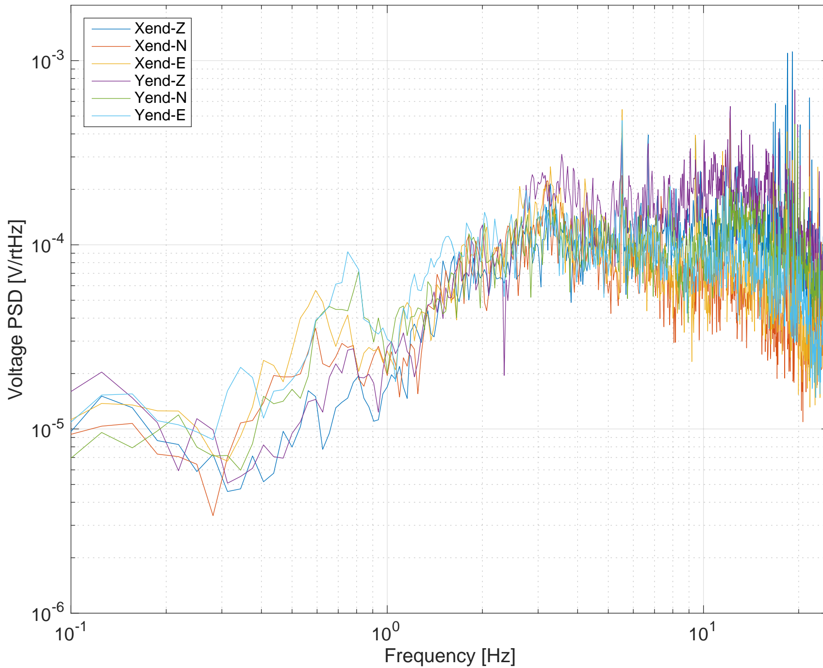
Raw voltage PSD: X/Yend guralp low vel output
