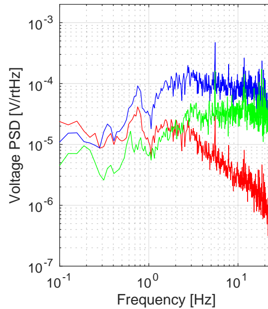
Raw voltage PSD: Yend guralp E
