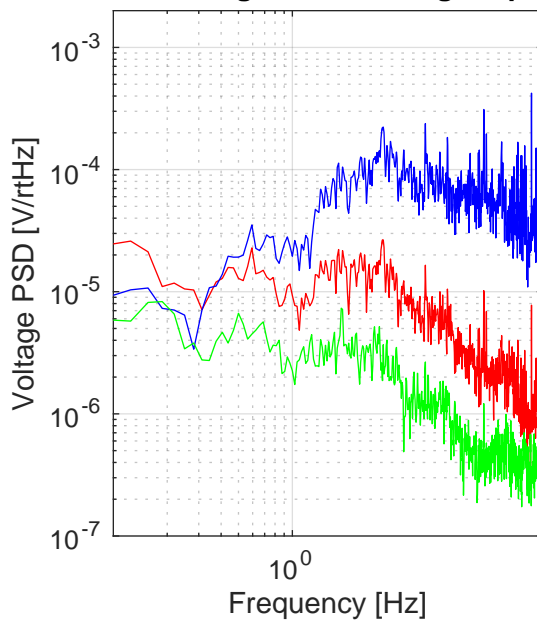
Raw voltage PSD: Xend guralp N
