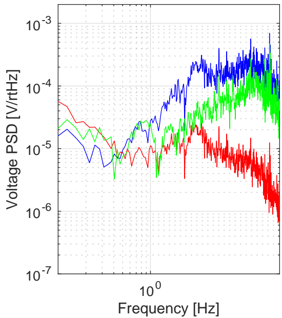
Raw voltage PSD: Yend guralp Z
