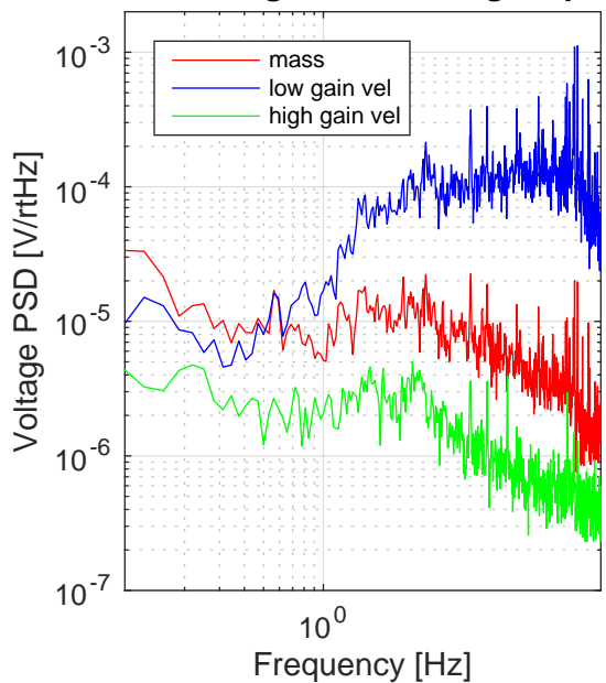
Raw voltage PSD: Xend guralp Z
