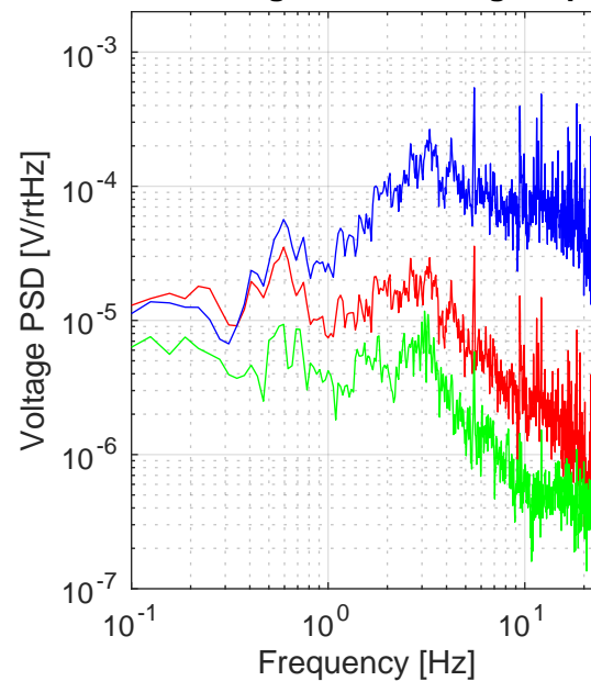
Raw voltage PSD: Xend guralp E
