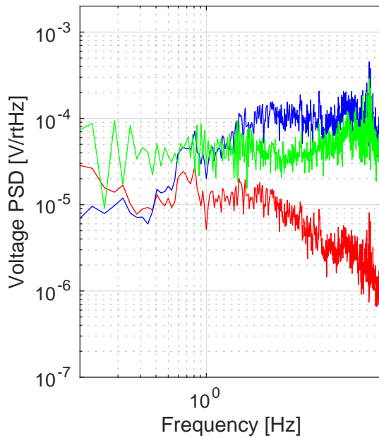
Raw voltage PSD: Yend guralp N
