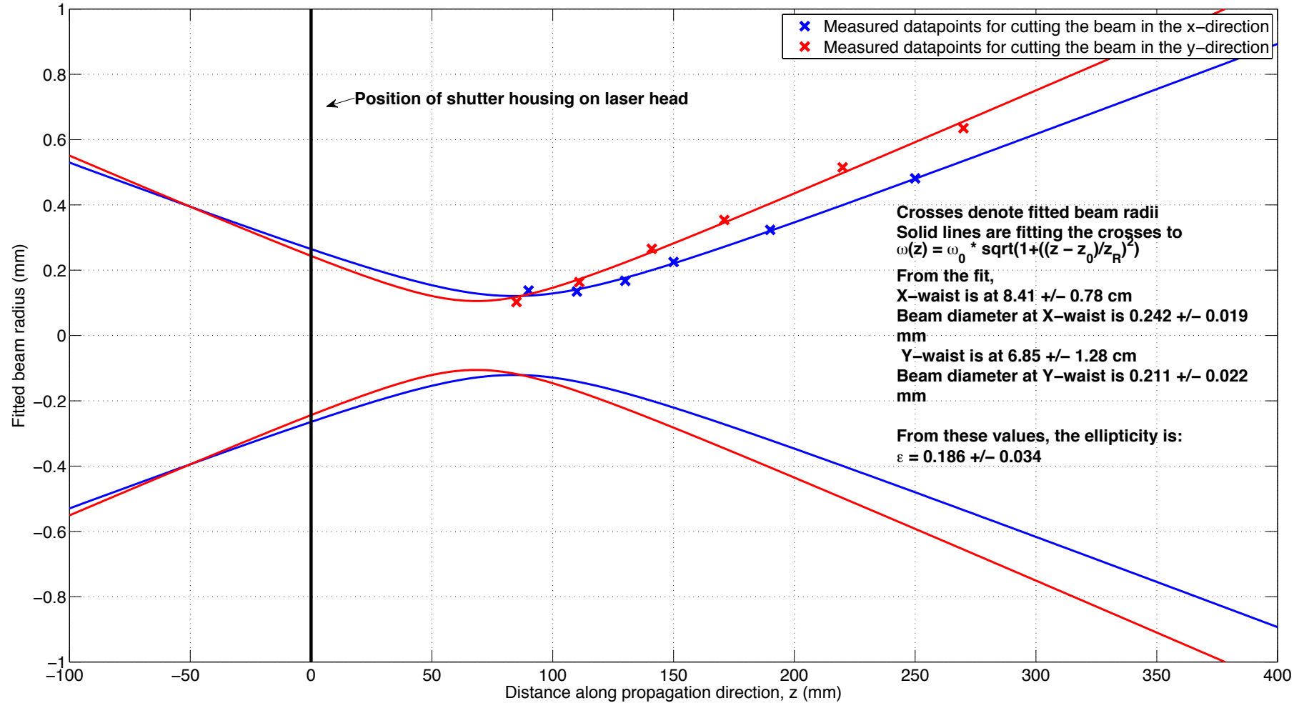
Beam profiling Lightwave NPRO: z-scan results
