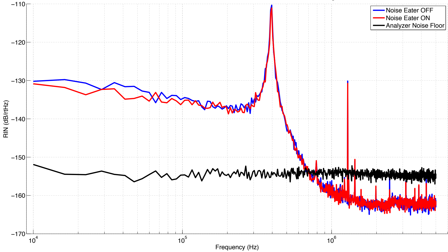
RIN measurement for AUX-X laser, I = 1.942A, T = 41.00 deg
