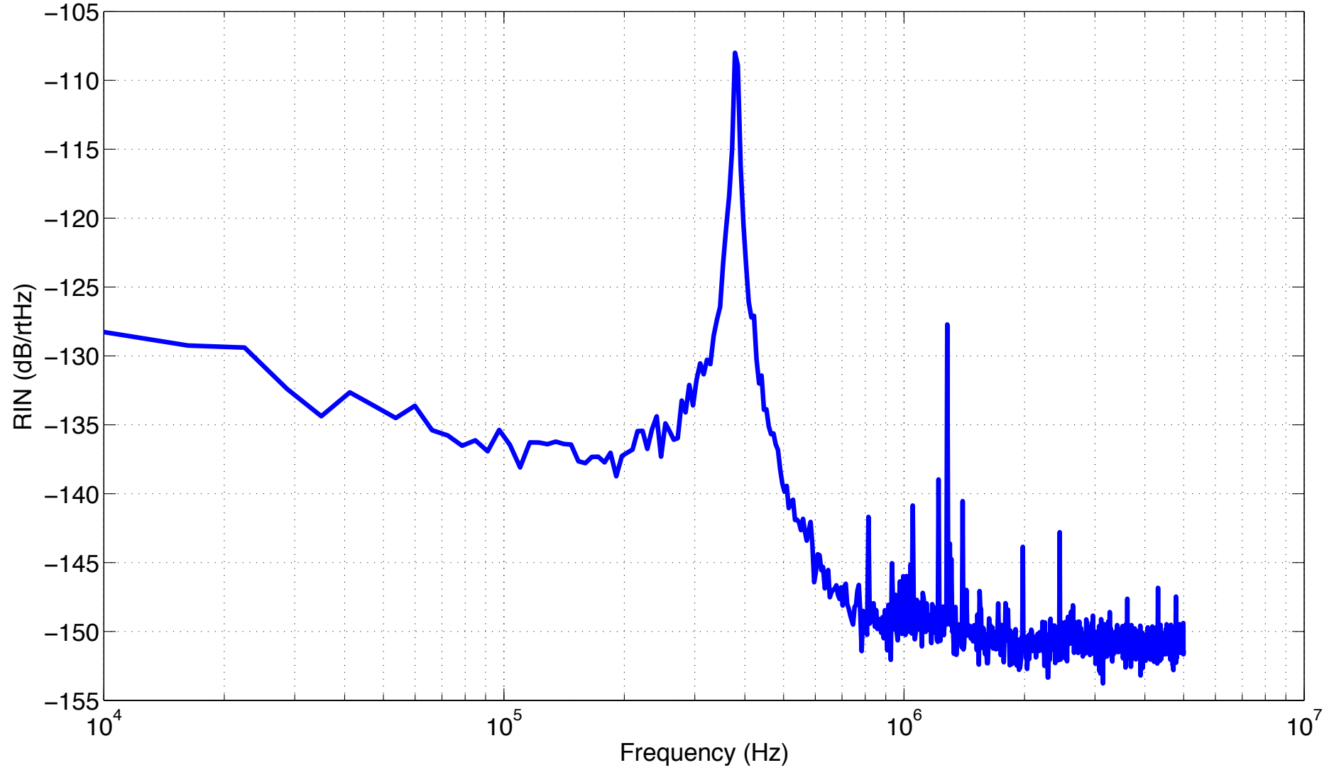
RIN measurement for AUX-X laser, I = 1.9A, T = 47.5 deg
