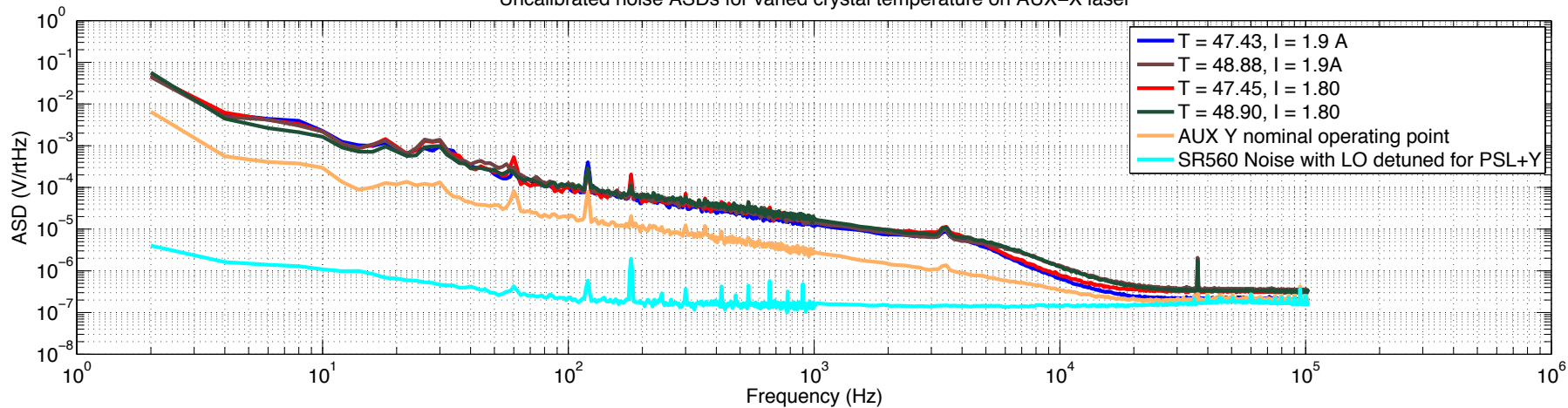
Uncalibrated noise ASDs for varied crystal temperature on AUX-X laser
