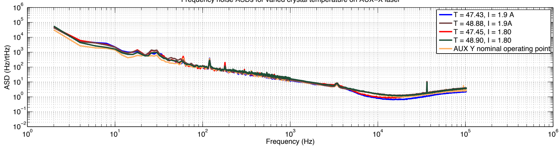
Frequency noise ASDs for varied crystal temperature on AUX-X laser
