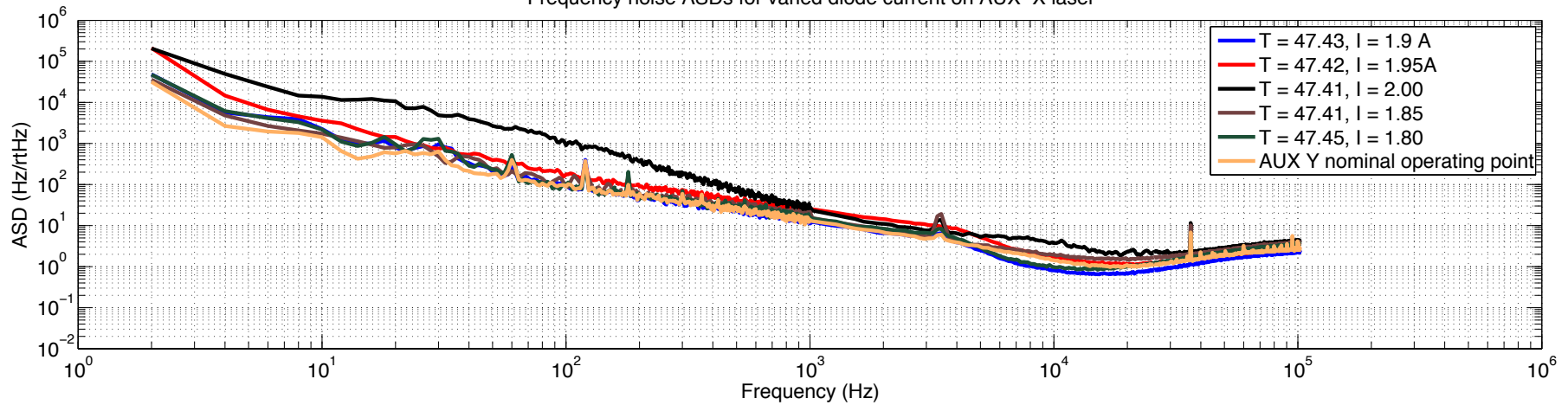
Frequency noise ASDs for varied diode current on AUX-X laser
