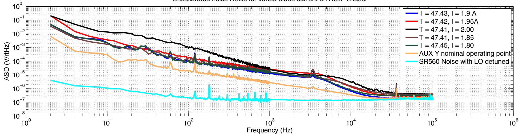
Uncalibrated noise ASDs for varied diode current on AUX-X laser
