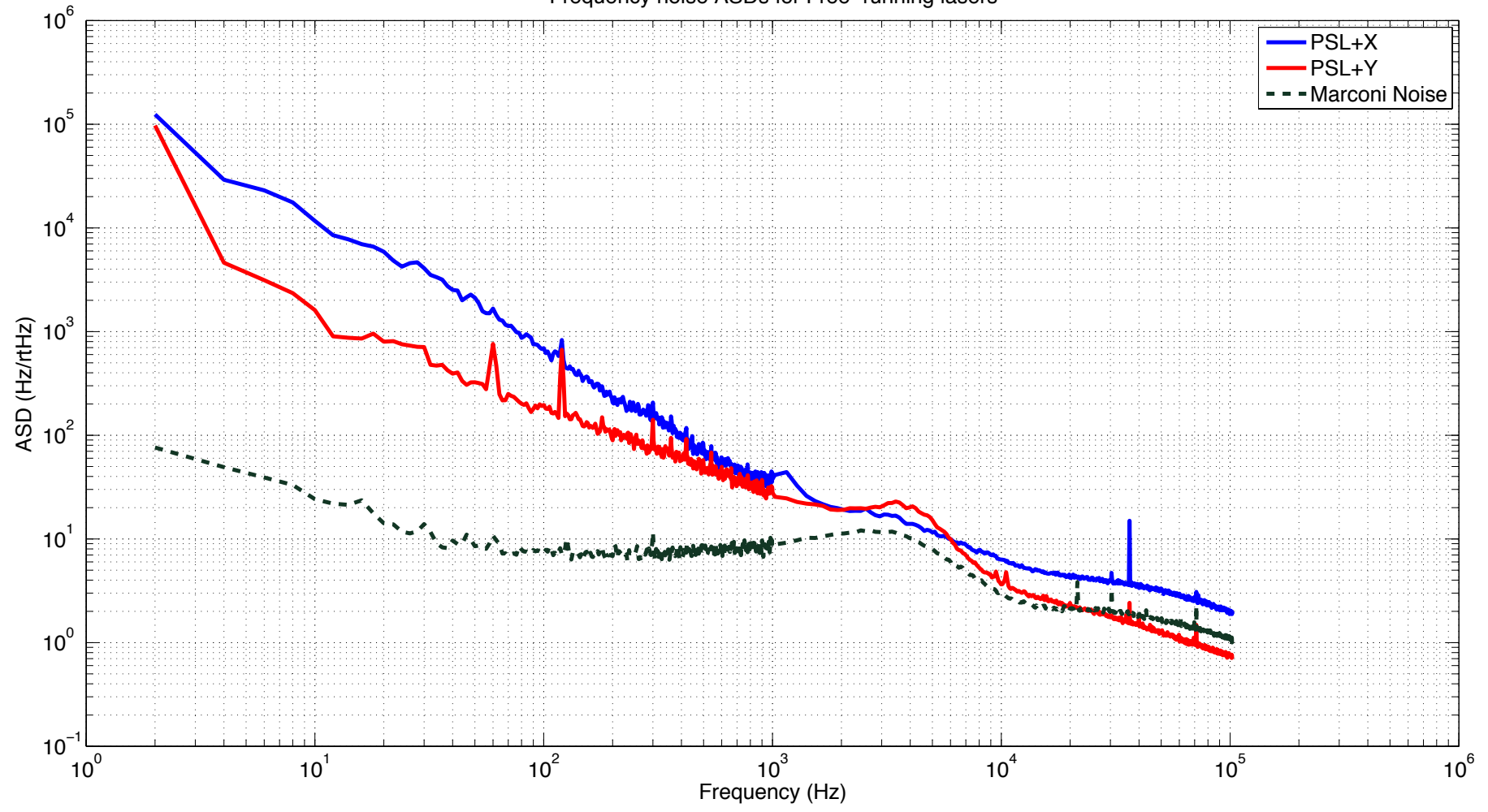
Frequency noise ASDs for Free-running lasers
