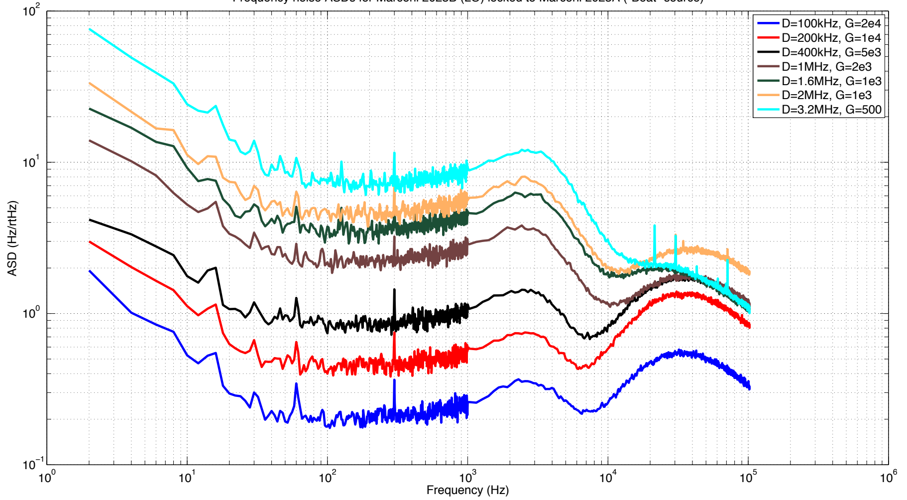
Frequency noise ASDs for Marconi 2023B (LO) locked to Marconi 2023A ("Beat" source)
