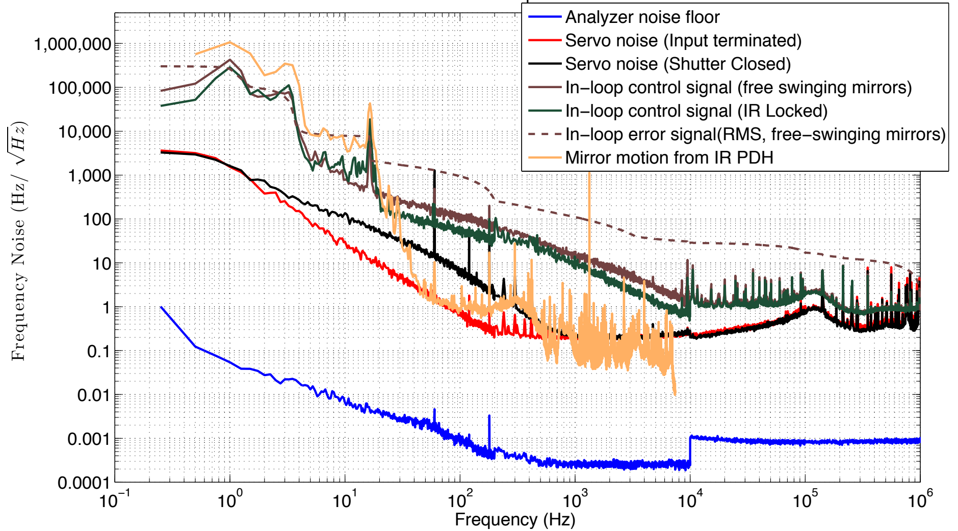
Y-arm AUX PDH loop noise breakdown
