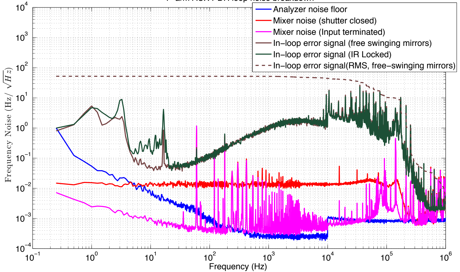
Y-arm AUX PDH loop noise breakdown
