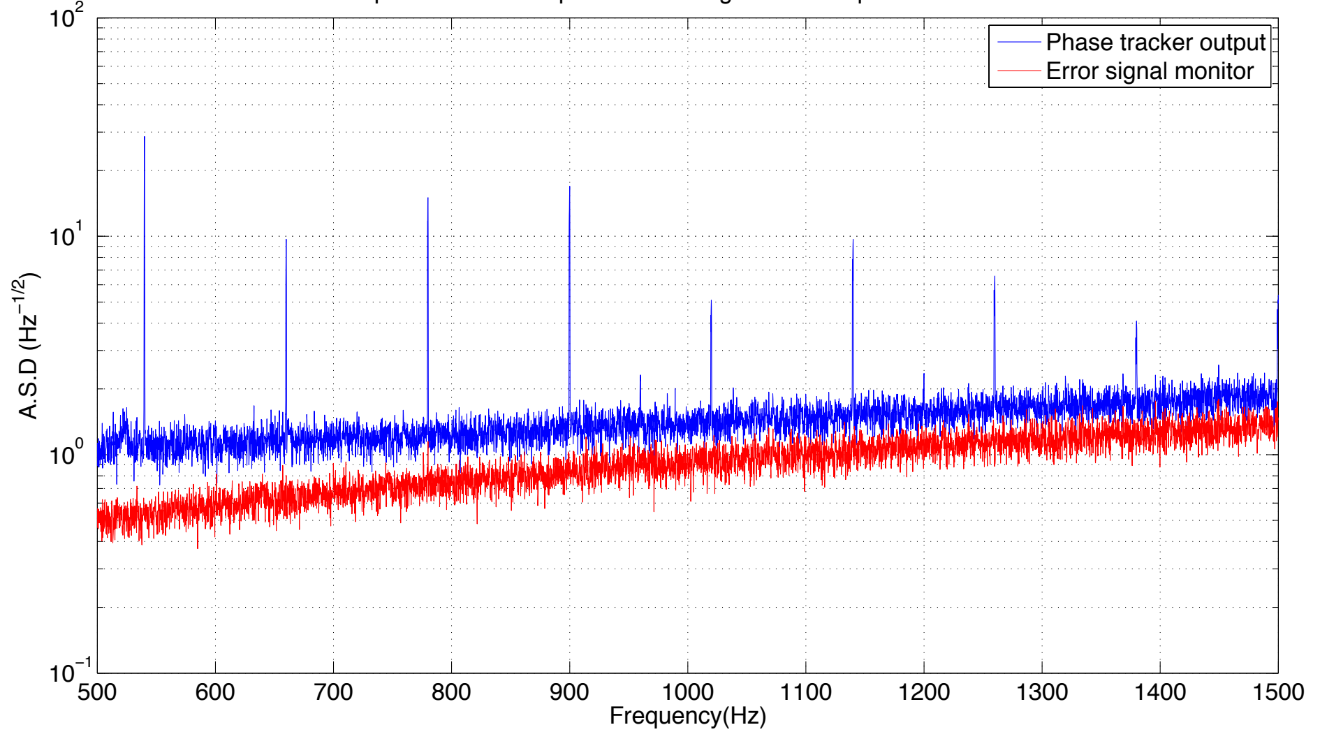
A.S.D of phase tracker output and error signal monitor point with no excitation
