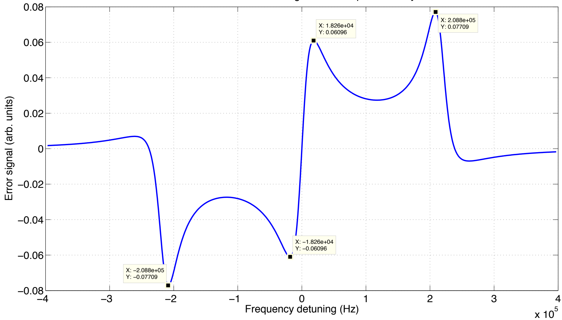
Simulated PDH error signal for a simple FP cavity
