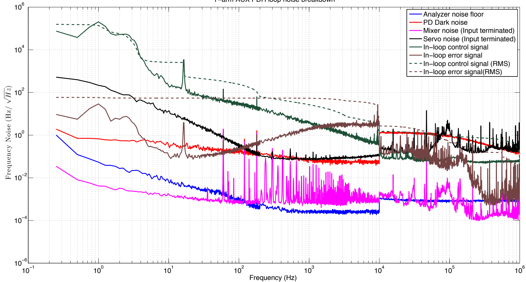
Y-arm AUX PDH loop noise breakdown
