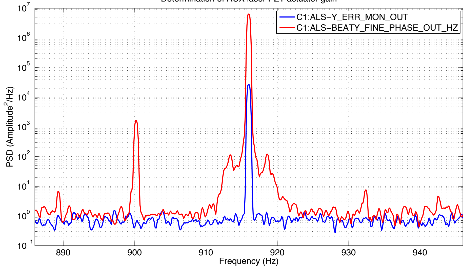
Determination of AUX laser PZT actuator gain
