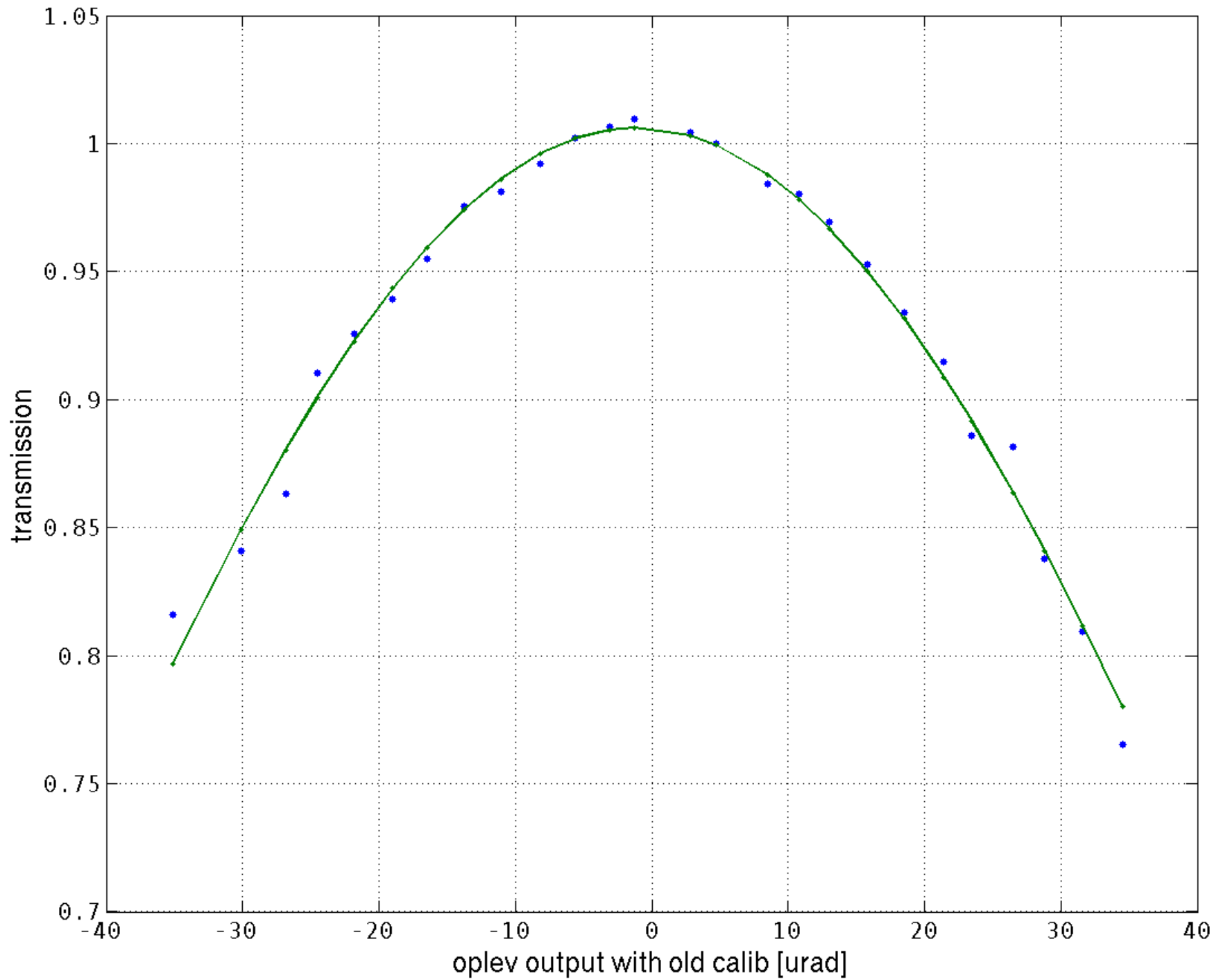
ITMY YAW
