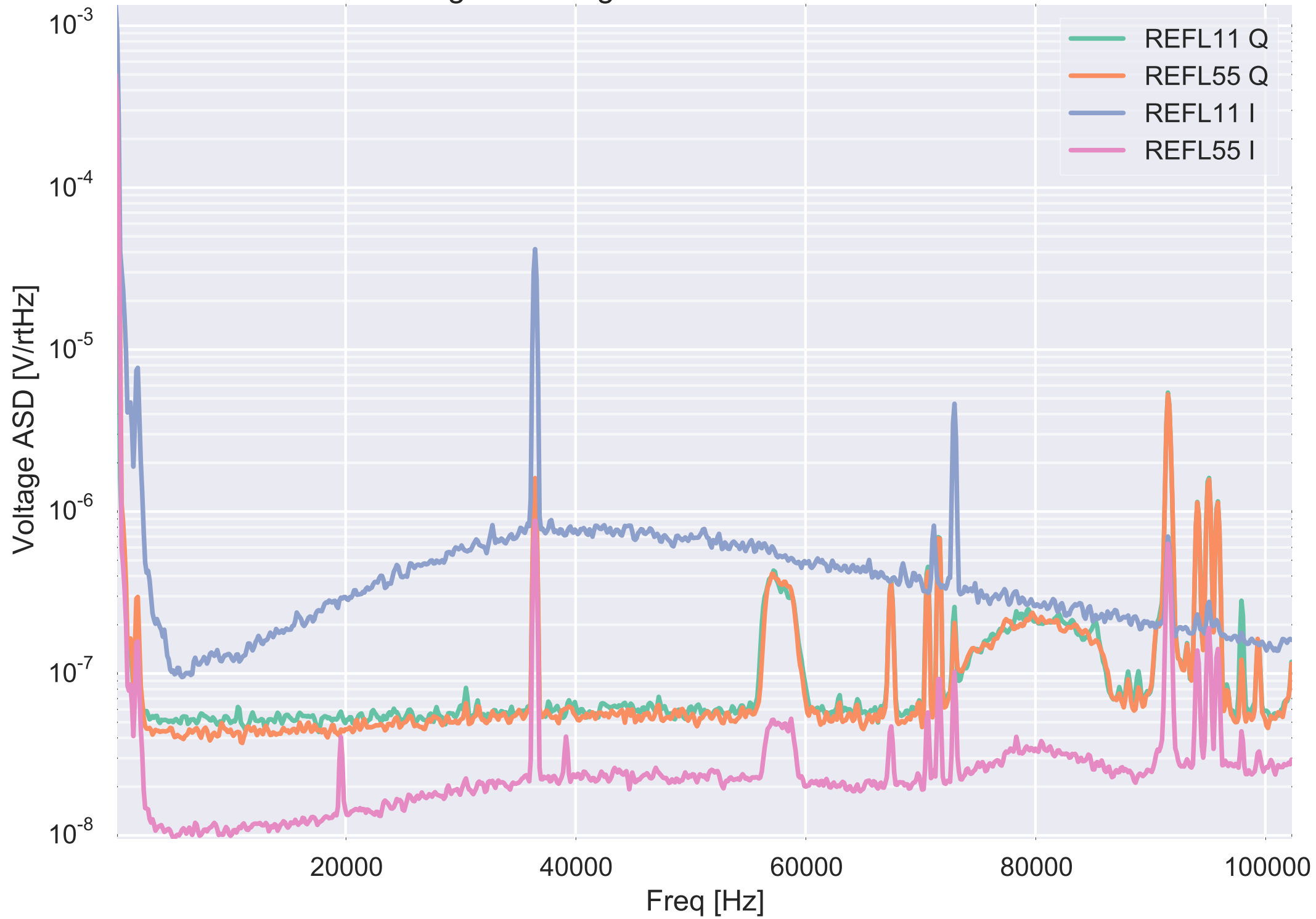
Analog RFPD Signals - PRMI Locked on Carrier
