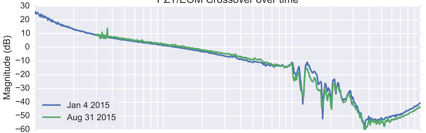
PZT/EOM Crossover over time
