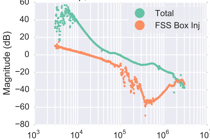
IMC Loop, Crossover Measurement
