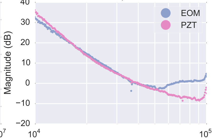
Inferred PZT, EOM Paths
