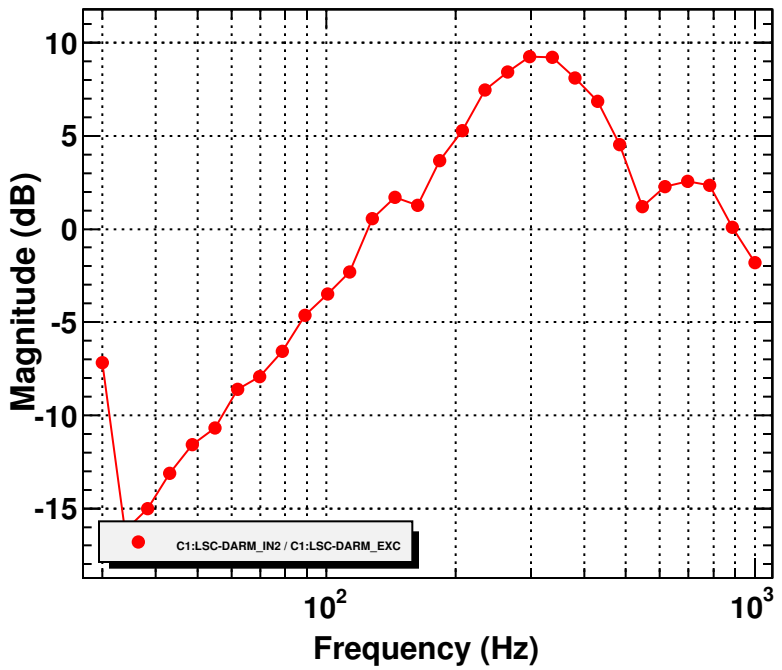
DARM A vs. B TF
