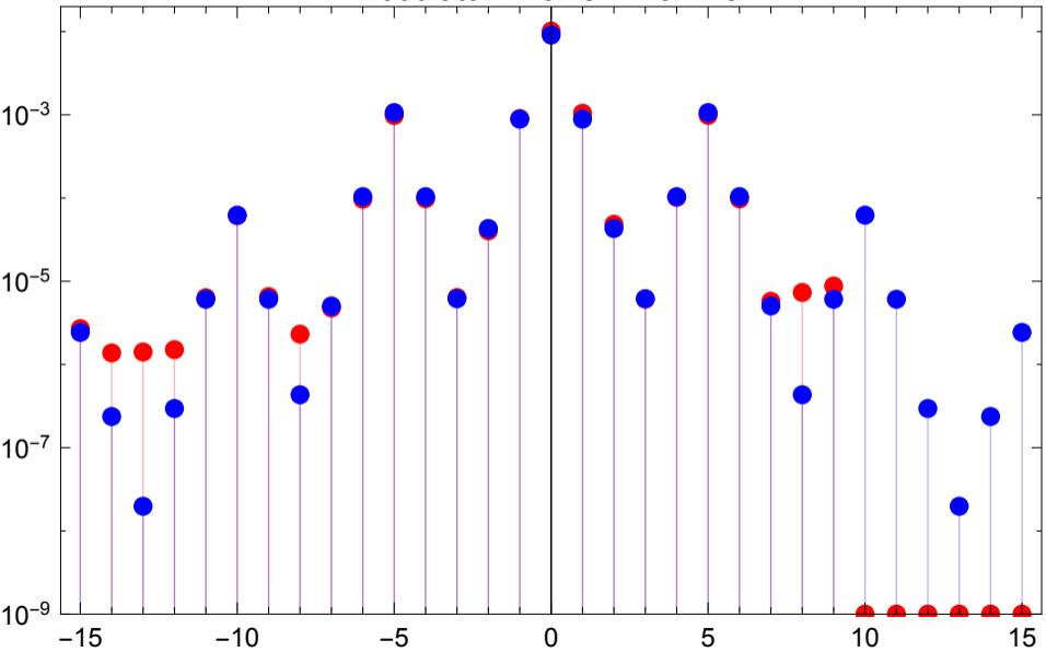
Modulaton Profile ~ Nominal
