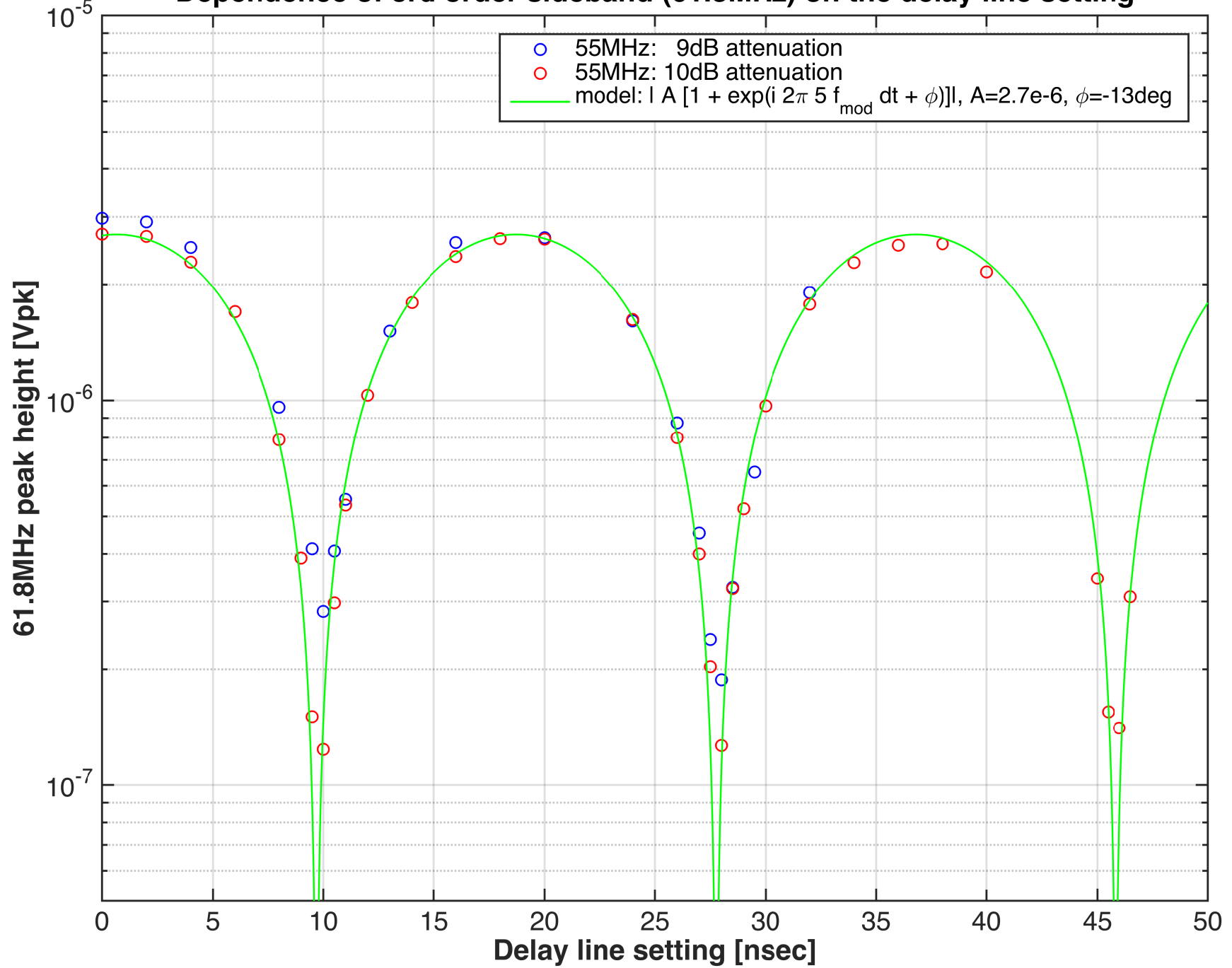
Dependence of 3rd order sideband (61.8MHz) on the delay line setting
