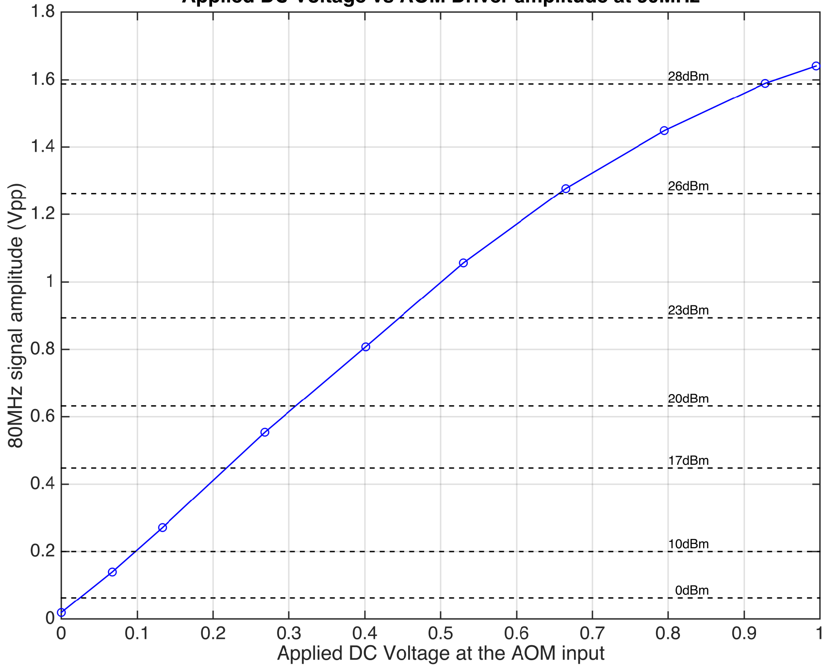
Applied DC Voltage vs AOM Driver amplitude at 80MHz
