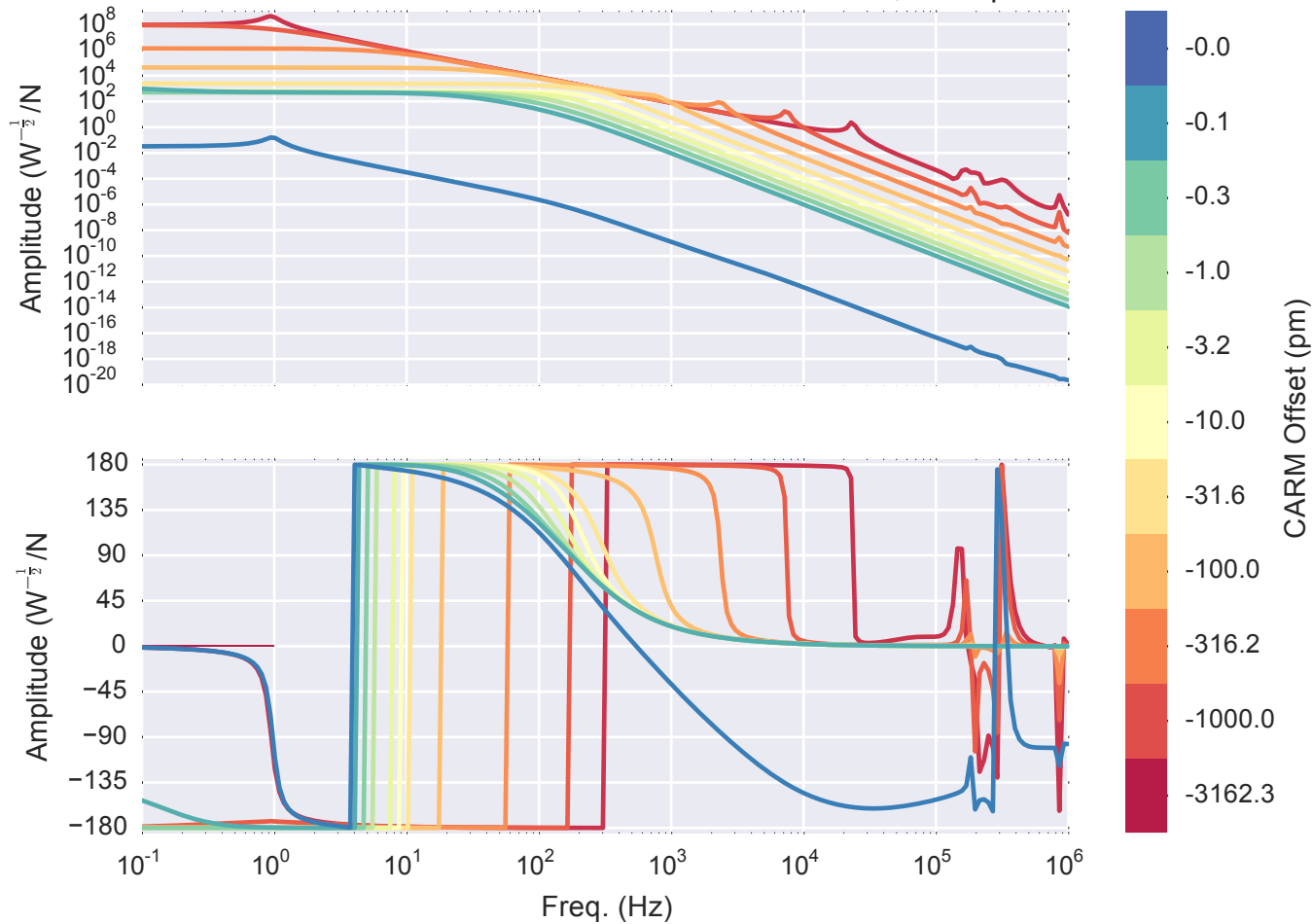
Carm to TRX -1/2 TFs with Radiation Pressure - PRMI, 1W input
